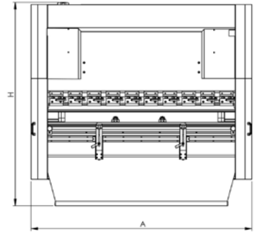
Model EB 1230 PARÇALI Üst Bıçaklıdır SEGMENTED 1250mm UPPER BLADE on Model EB 1230
