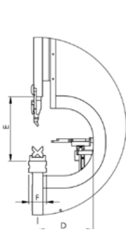
Model EB 1540 / EB 2160 Üst Bıçaklar Parçalıdır. Segmented Upper Blades on Model EB 1540 / EB 2160
