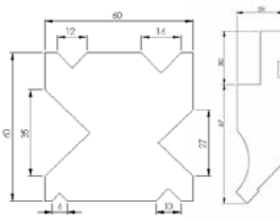
Model EB 1230 PARÇALI Üst Bıçaklıdır SEGMENTED 1250mm UPPER BLADE on Model EB 1230
