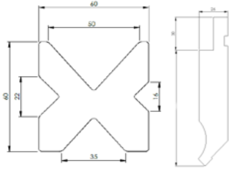
Model EB 1540 / EB 2160 Üst Bıçaklar Parçalıdır. Segmented Upper Blades on Model EB 1540 / EB 2160
