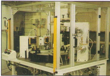
Light Curtain Mounting Bracket and Guard Combination Around Assembly Machine
