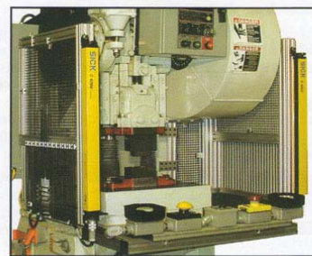
Point-of-Operation Light Curtains on a Press
