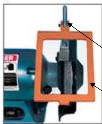
Adjustable locks
